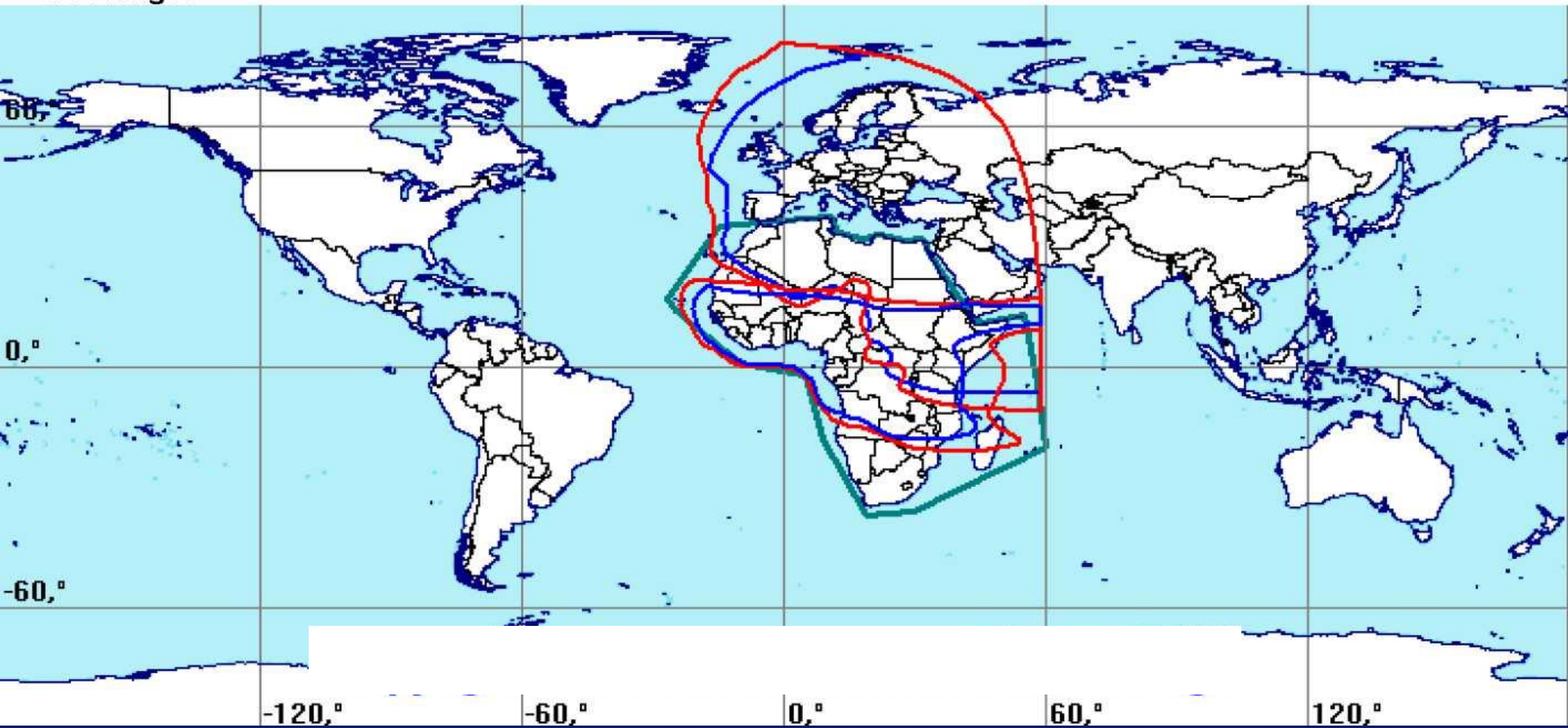
Figure 101 : Ku Band Europe / Africa coverage on satellite SES-4
